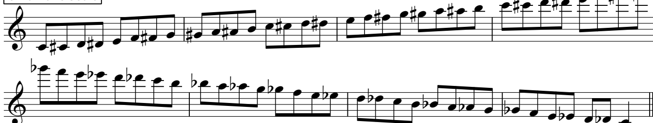
Chromatic Scale
